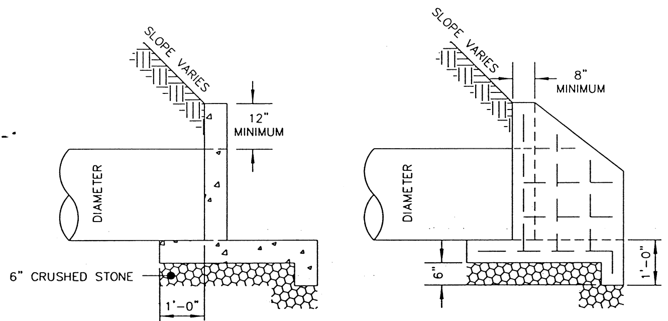
CROSS SECTION
