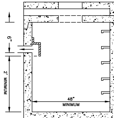
SECTION - CURB INLET
