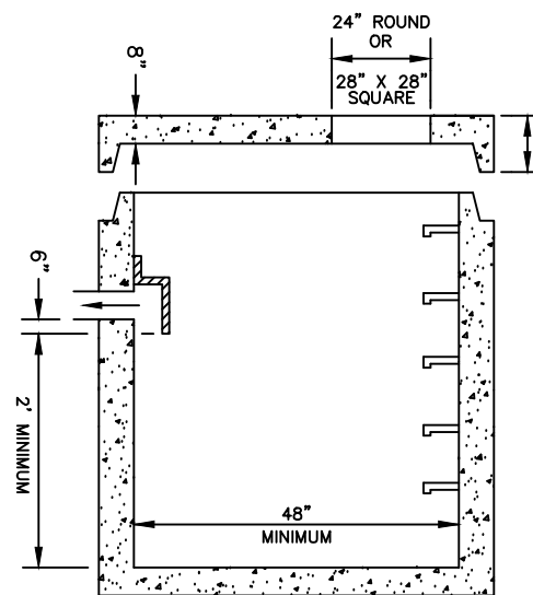
SECTION - FLAT TOP
